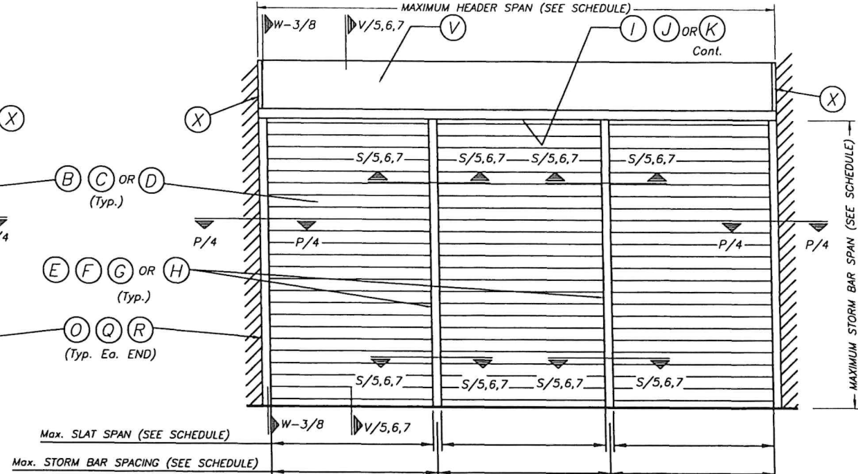
TYPICAL MULTIPLE UNIT ELEVATION (STORM BARS REQUIRED) NOTE: SEE SHEET 2 & 3 OF 13 FOR COMPONENTS NOMENCLATURE.
