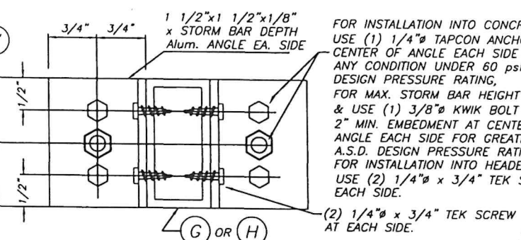
SECTION S - S (FOR FIXED STORM BAR) SCALE: 1/2" = 1"
