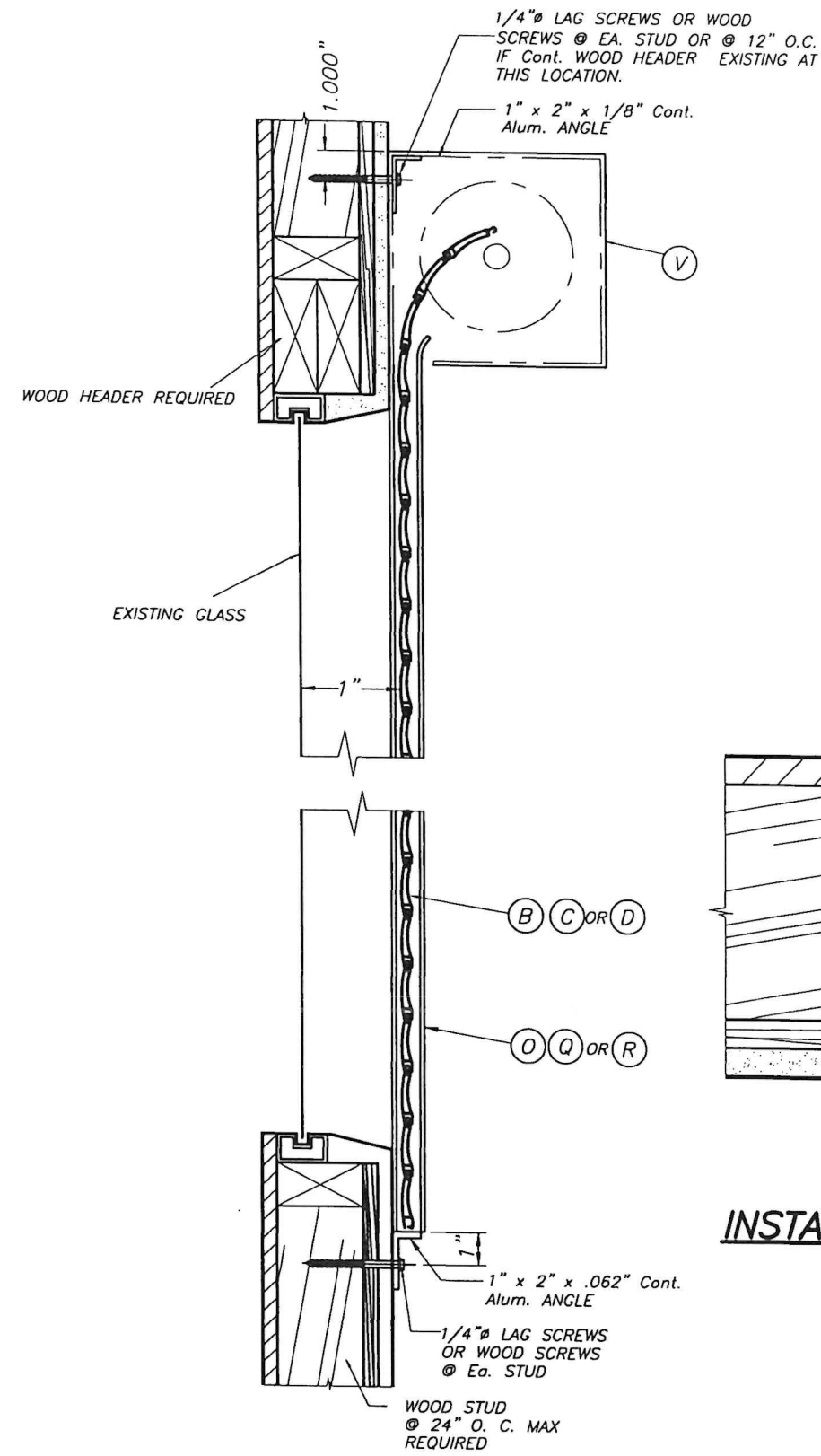
WALL MOUNTING INSTALLATION SINGLE SPAN CONDITION N. T. S.
