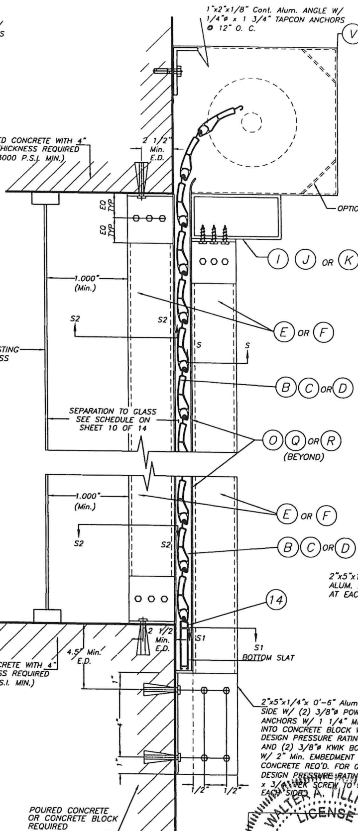
WALL MOUNTING: SECTION V-V(1) INSTALLATION W/ FIXED STORM BARS W/ CONCRETE ANCHORS SCALE: N.T.S.
