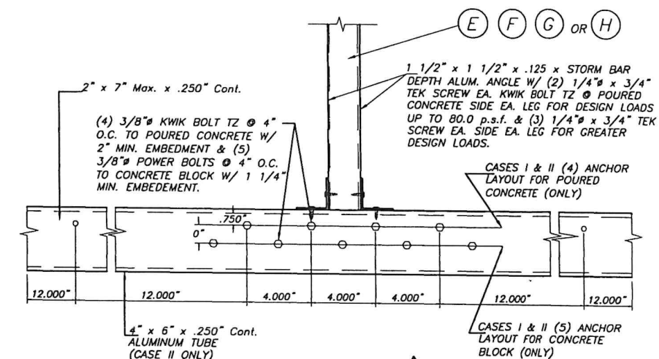
ELEVATION X
