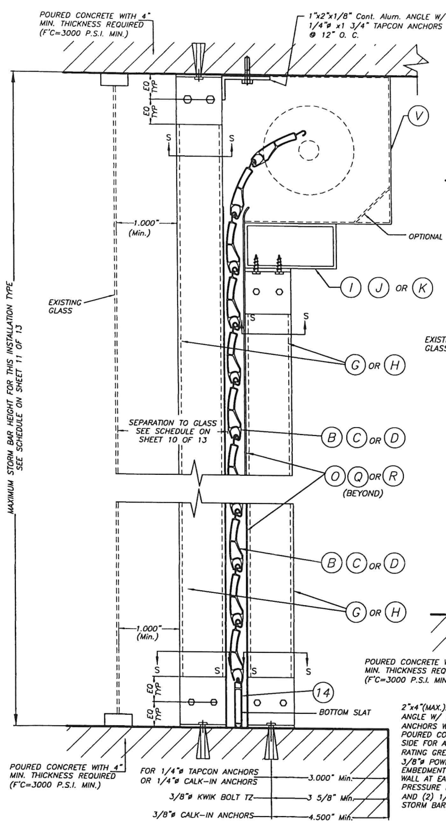
CEILING & FLOOR MOUNTING: SECTION V-V(2) INSTALLATION W/ FIXED OR REMOVABLE STORM BARS W/CONCRETE ANCHORS (SEE SECTION S-S FOR ANCHOR TYPE REQUIREMENT) N.T.S.
