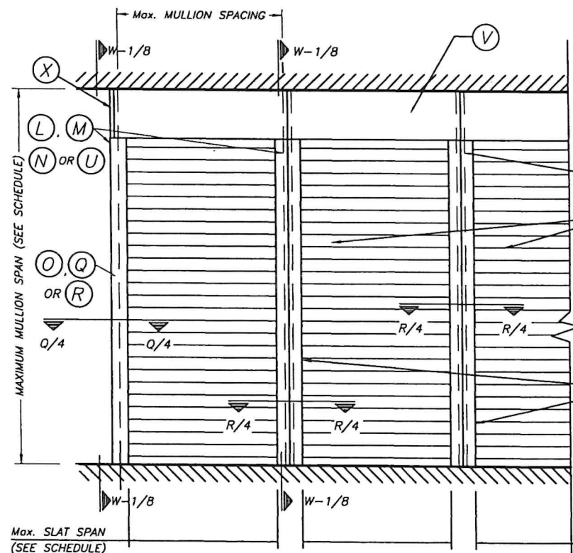
TYPICAL CONSECUTIVE SINGLE UNIT ELEVATION (NO STORM BARS REQUIRED) NOTE: SEE SHEET 2 & 3 OF 13 FOR COMPONENTS NOMENCLATURE.
