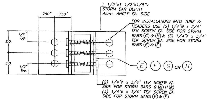
SECTION S3 - S3
