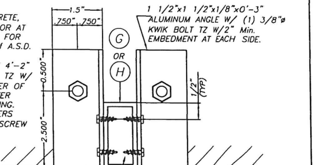
SECTION S2 - S2 SCALE: 1/4" = 1"
