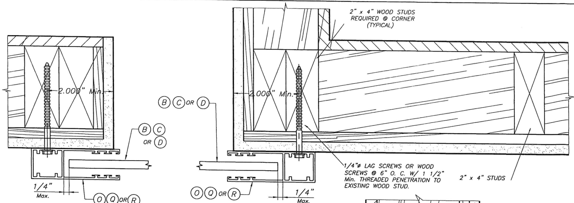
PLAN A (SECTION) WALL MOUNT SCALE : 3/8" = 1"
