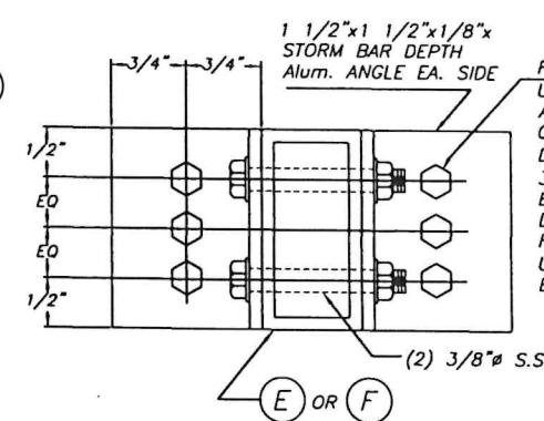
SECTION S - S (FOR REMOVABLE STORM BAR) SCALE: N.T.S.
