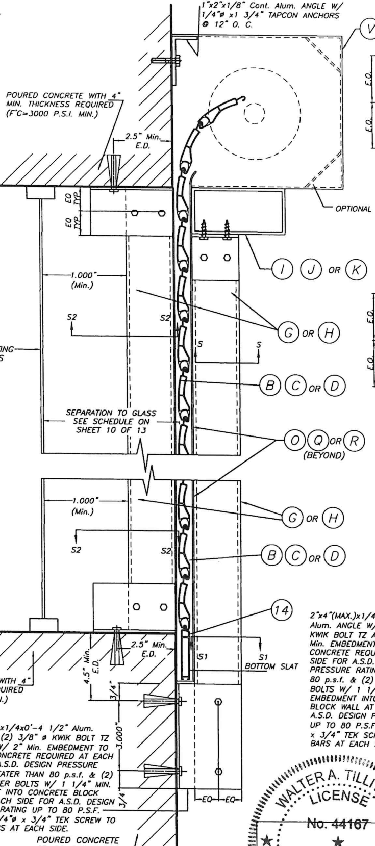
WALL MOUNTING: SECTION V-V(1) INSTALLATION W/ FIXED STORM BARS W/CONCRETE ANCHORS N.T.S.
